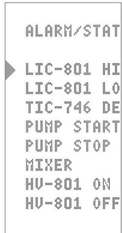
Figure 8: Alarm/Status Display
