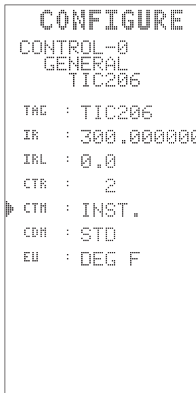
Figure 11: Control Loop Configuration
