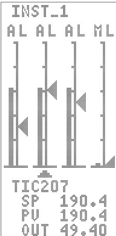
Figure 6: Four Loop Display
